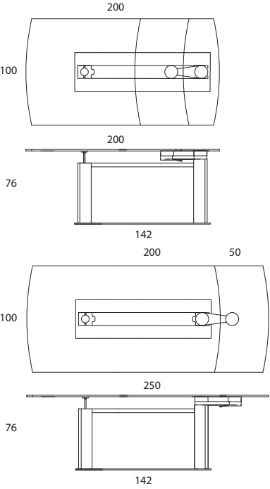
Cod.593+029 L200+50xP100xH75 Tavolo allungabile / Extendible table /Table extensible
