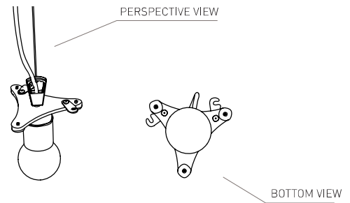
FLORA SUSPENSION S 1 X E26 BULBS MagneticSystem®
